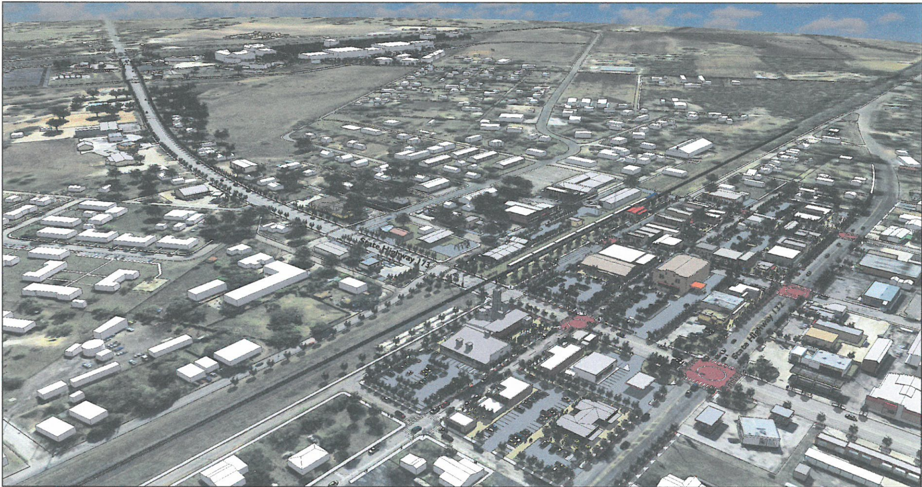
Figure 51: Proposed Improvements along Texas State Highway 173
